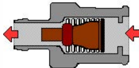
PCV Valve Minimum flow at idle/low speed
