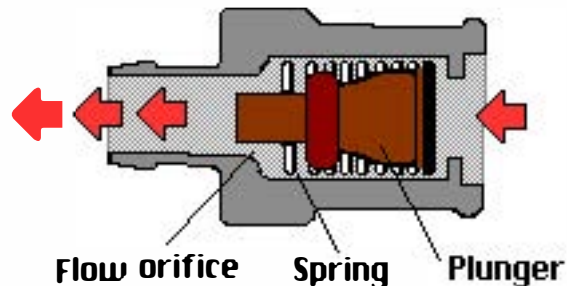
Maximum flow at high speed/load
