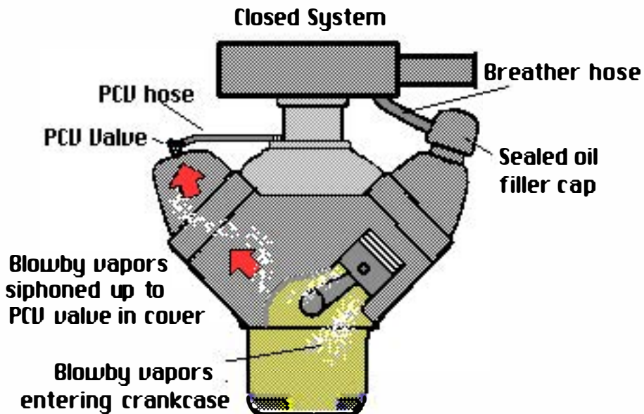
Maximum flow at high speed/load
